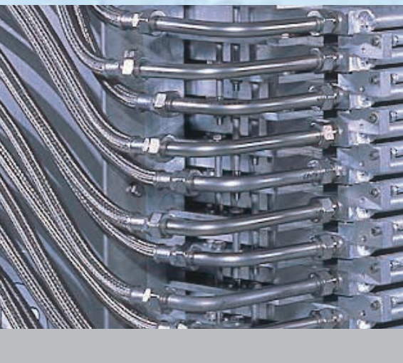
Flexible PTFE hoses, for freon, stainless steel-armoured individually pressure tested. Stainless steel bellow hoses for R717, individually pressure tested. Stainless steel fittings.
